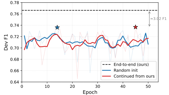
Figure 7: Per-epoch dev F1 under two initializations on Re-DocRED. Faint lines show raw F1. Bold lines show the 5-epoch moving average. Stars mark each setting’s best epoch. The dashed line marks our full model performance (F1=0.7663).
